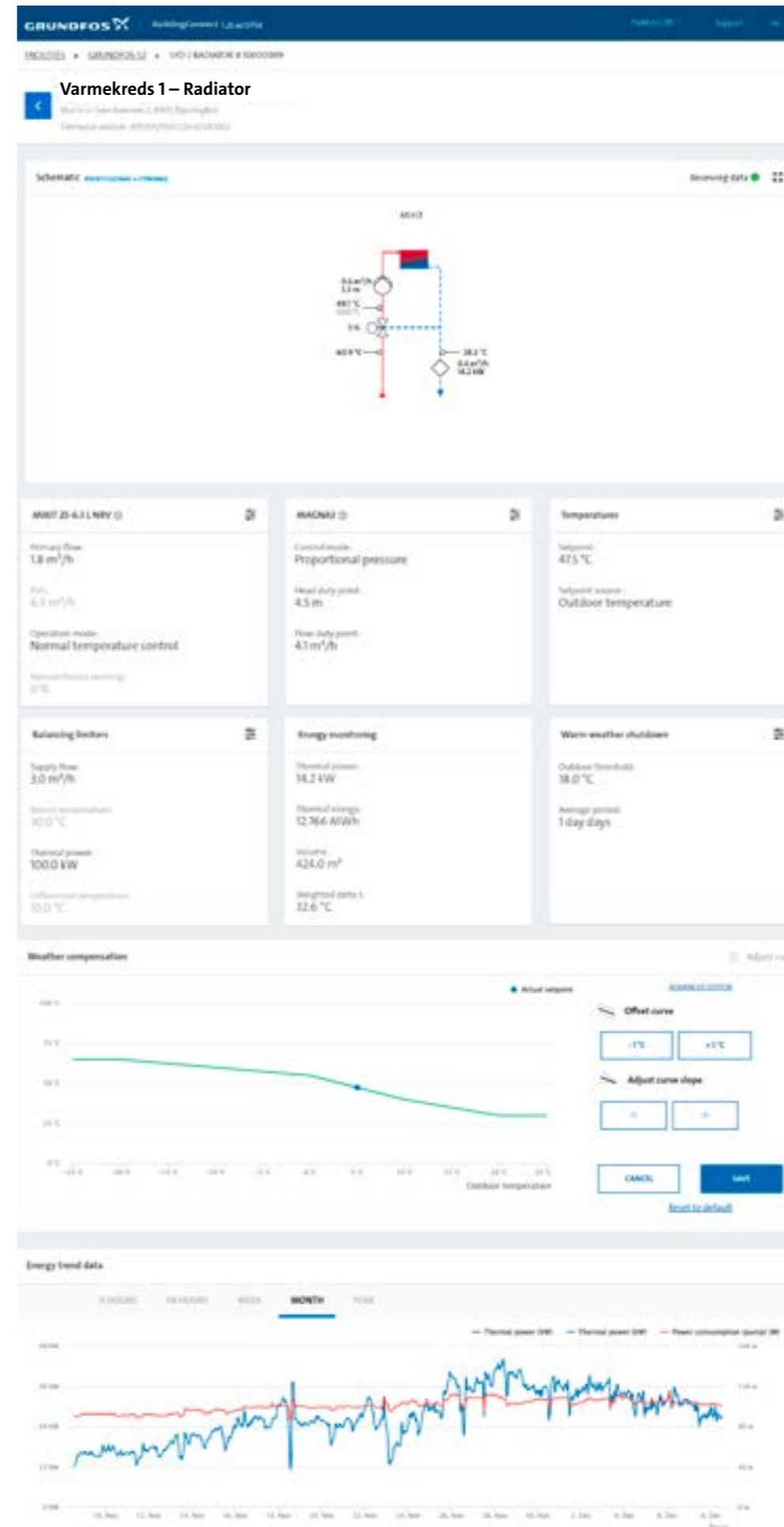
Illustration af MIXIT Dynamic-dashbordet i BuildingConnect:
