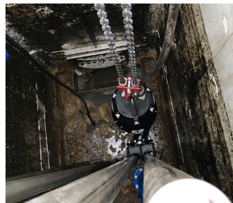
The Grundfos 18.5 kW SL pumps are wet installed in the pumping station.
